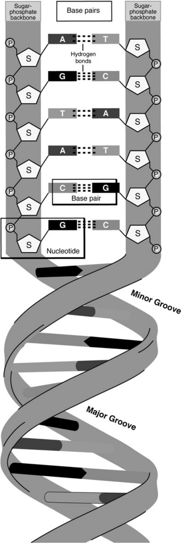
Figure 2. DNA
